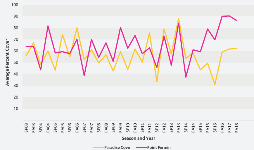
Surfgrass Populations ( Phyllospadix , spp.) in Los Angeles County (2003 – 2018)
