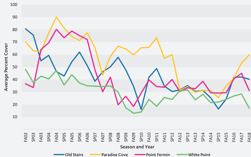
Acron Barnacle Populations ( Chthamalus fissus/dalli and Balanus glandula ) in Los Angeles County (2002-2018)
