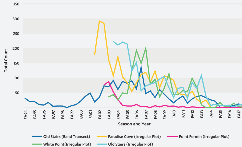
Ochre Sea Star Populations ( Pisaster ochraceus ) in Los Angeles County (1994 – 2017)
