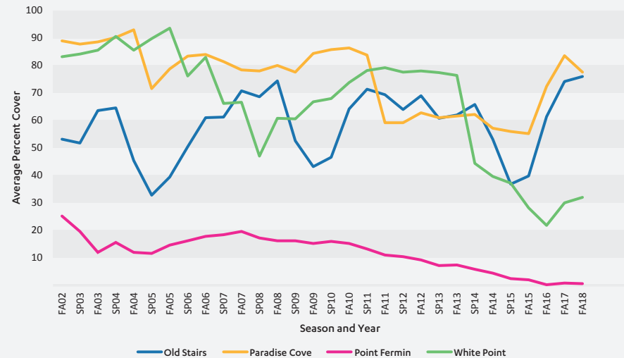
California Mussel Populations ( Mytilus californianus ) in Los Angeles County (2002-2018)
